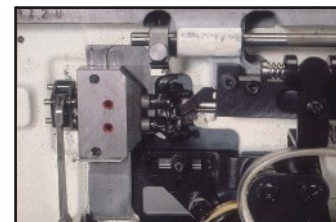
Looper assembly
